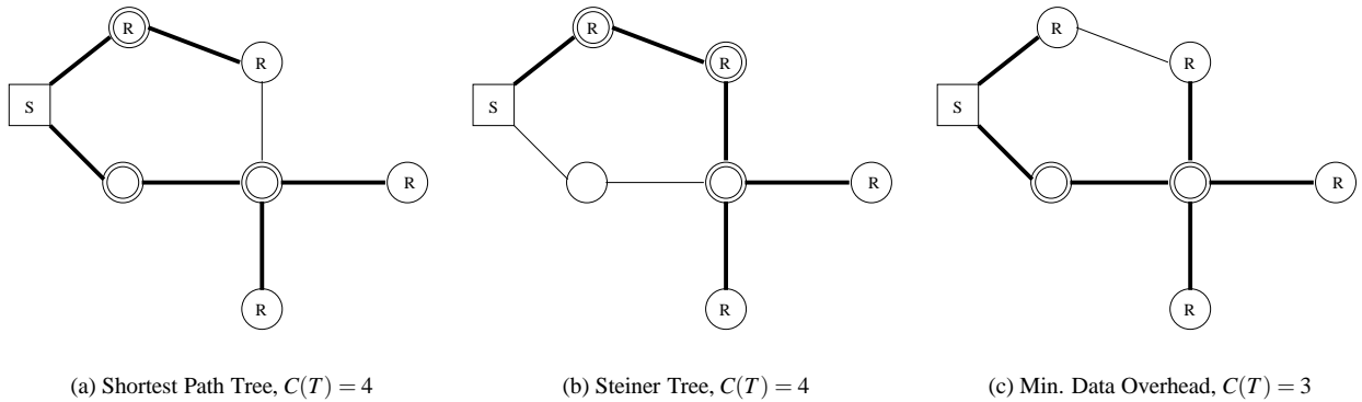
Fig. 2. Differences in cost for several multicast trees over the same ad hoc network
