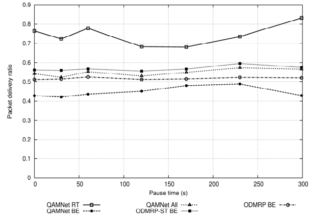
Figure 6. Packet Delivery Ratio as a function of pause time.
