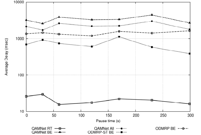
Figure 5. Average Delay in msec as a function of pause time.
