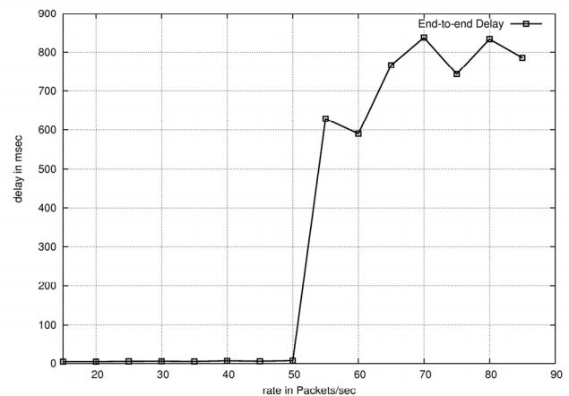
Figure 2: End-to-End Delay as function of traffic load
