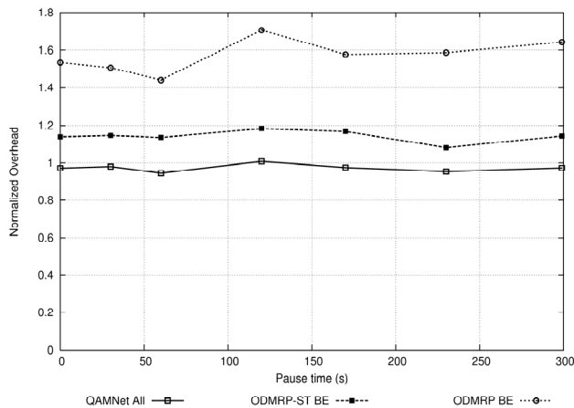
Figure 7. Normalized Overhead as a function of pause time.
