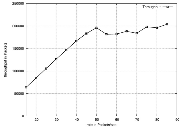
Figure 1: Throughput as function of offered traffic load
