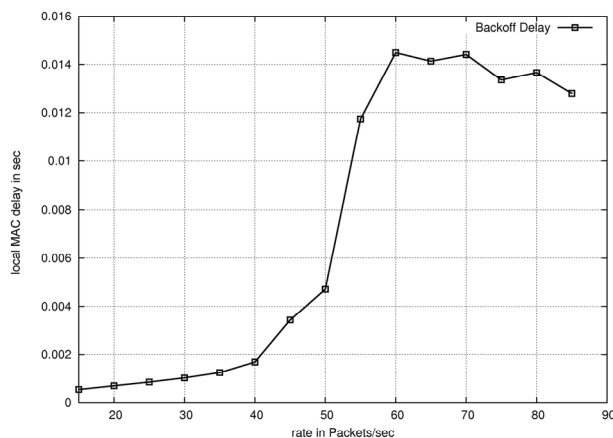
Figure 4: Local nodes MAC backoff delay as function of offered traffic load
