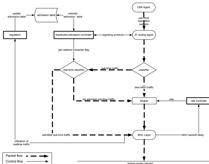
Figure 3: QAMNet Architecture within MANET nodes
