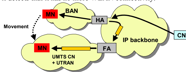
Figure 2 Vertical handover with no coupling between WLAN and UMTS
