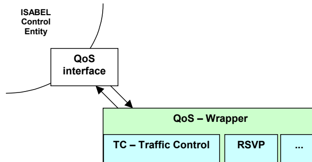
Figure 6. QoS wrapper
