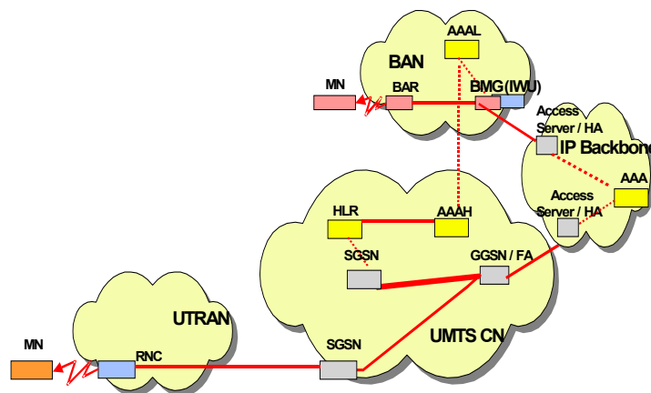
Figure 3. Vertical handover with loose coupling between WLAN and UMTS
