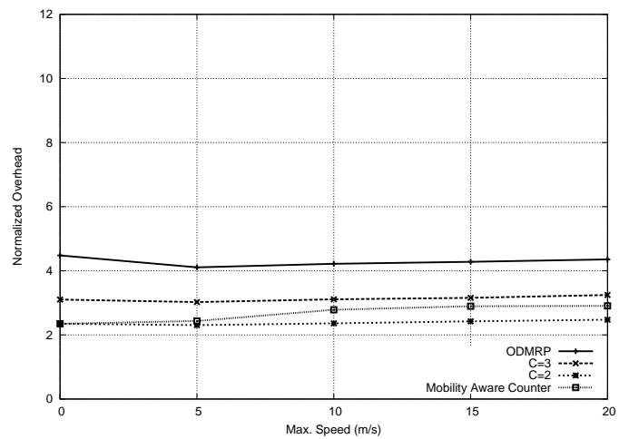
Fig. 8. Overhead with 2 sources and 15 receivers
