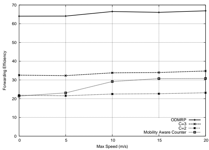
Fig. 12. FEF with 4 sources and 15 receivers
