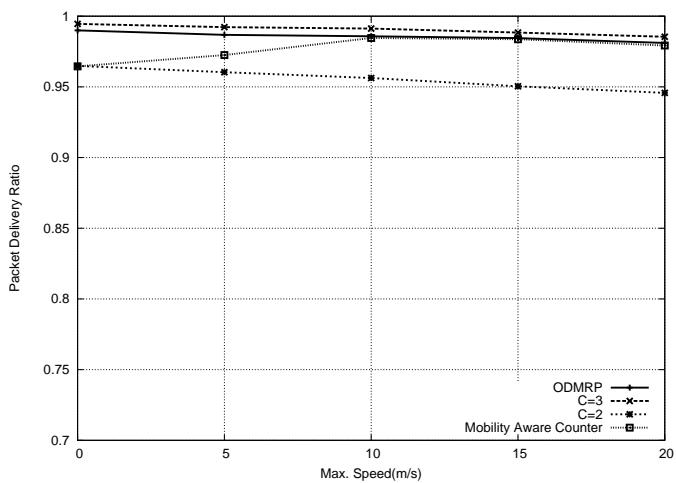
Fig. 6. PDR with 4 sources and 15 receivers
