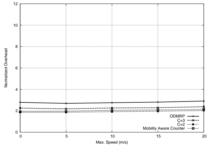
Fig. 7. Overhead with 1 source and 15 receivers
