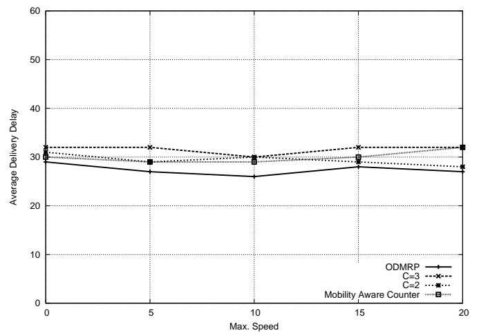
Fig. 14. Average Delivery Delay with 2 sources and 15 receivers
