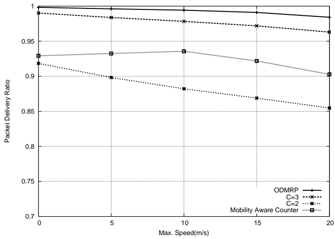
Fig. 4. PDR with 1 source and 15 receivers
