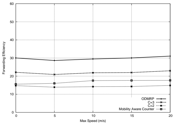
Fig. 10. FEF with 1 source and 15 receivers
