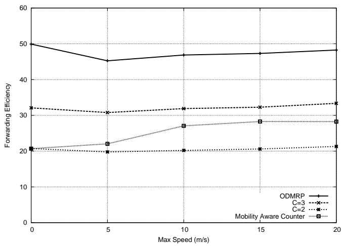
Fig. 11. FEF with 2 sources and 15 receivers
