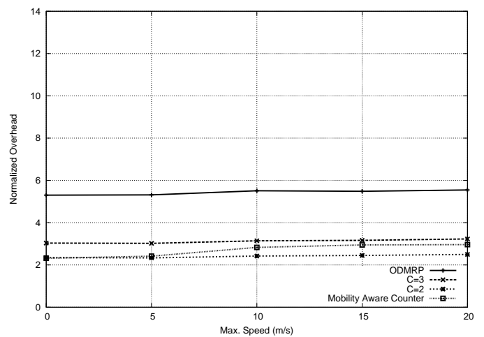
Fig. 9. Overhead with 4 sources and 15 receivers
