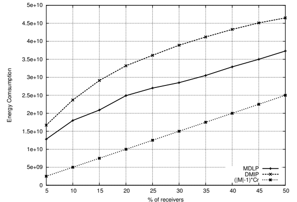
Figure 6: Energy consumed as a function of the percentage of receivers nodes with a network density of 500 \text{ nodes}/\text{Km}^2
