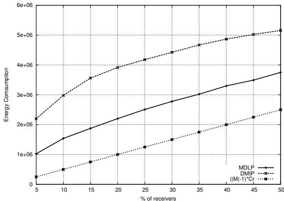
Figure 6: Energy consumed as a function of the percentage of receivers nodes with a network density of 500 \text{ nodes}/\text{Km}^2
