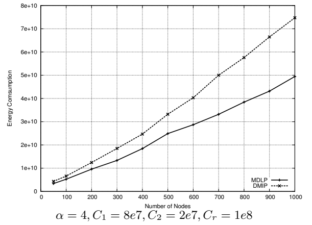
Figure 5: Energy consumed as a function of network density with 20% of receivers.
