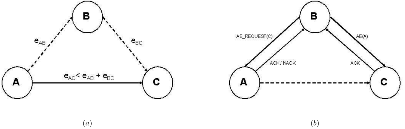
Figure 3: Example which shows the autoExcluding of node B.
