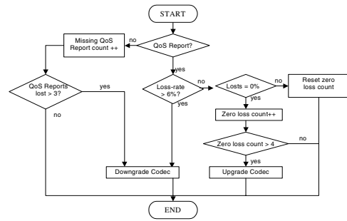
Fig. 2. Diagram of the initial adaptation logic used
