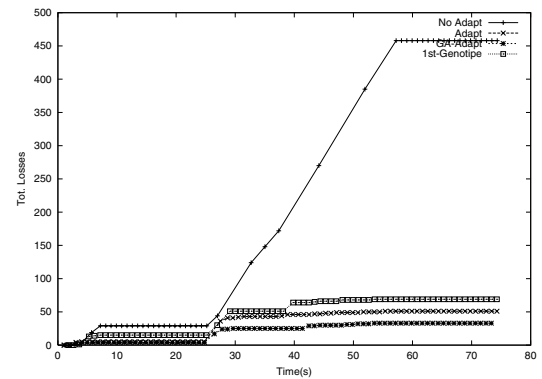
Fig. 5. Total packet losses with the different behaviours
