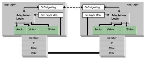
Fig. 1. Overall adaptation architecture
