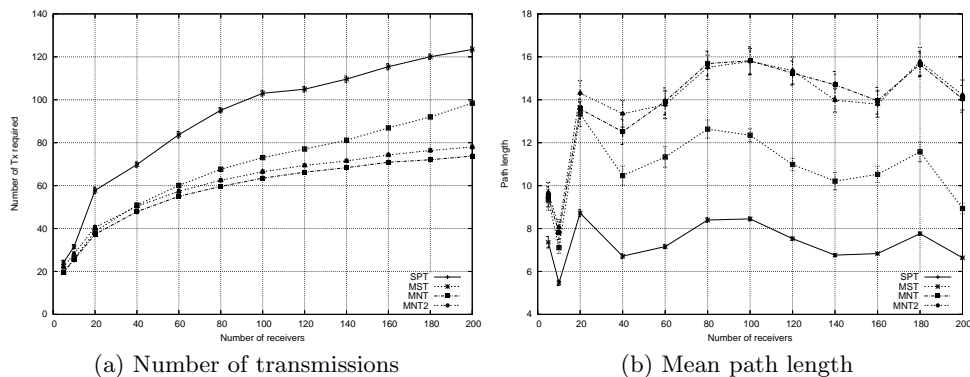
Fig. 3. Number of Tx and mean path length at increasing number of receivers.
