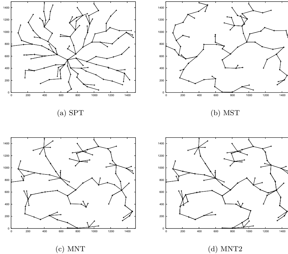
Fig. 2. Shape of example trees produced by heuristics
