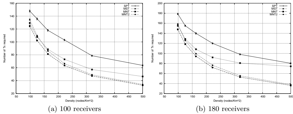
Fig. 4. Number of Tx with varying network density
