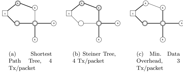
Fig. 1. Differences in cost for several multicast trees over the same ad hoc network
