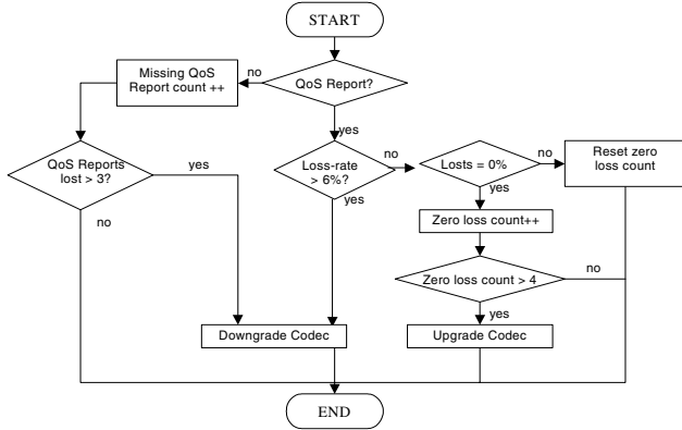
Fig. 5. Schematic diagram of the adaptation logic
